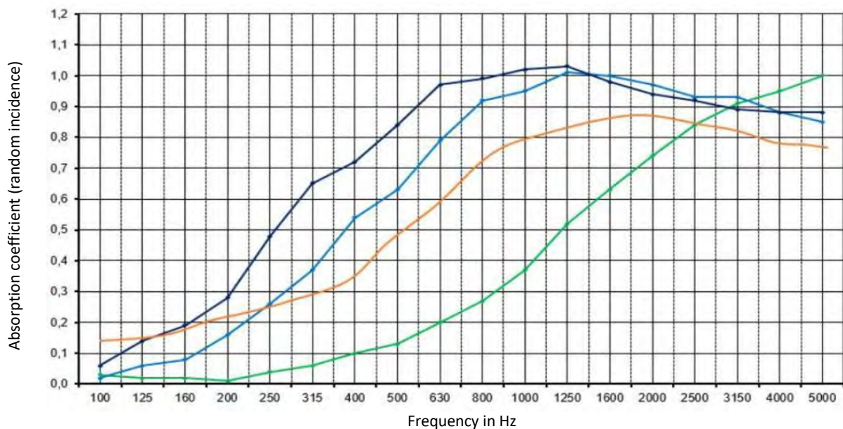
Measurement of sound absorption in a reverberation room (ISO 354:2003/ISO 11654)
